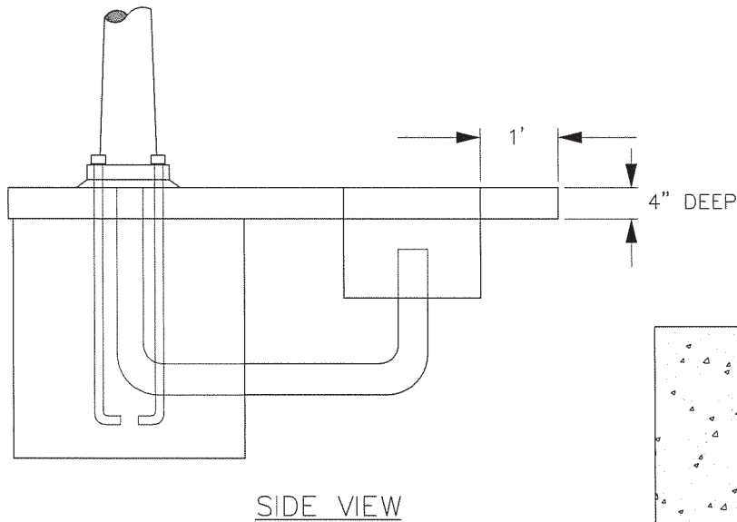
LIGHTING STANDARD & JUNCTION BOX
