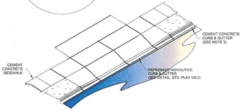
TYPE R1B - ISOMETRIC VIEW (RESIDENTIAL, WITH BUFFER)
